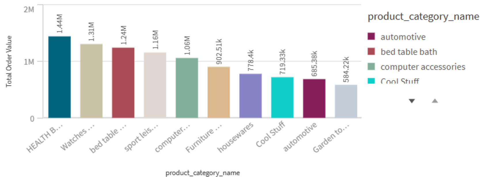
Top 10 Categories
